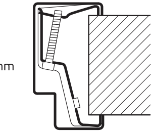
Wandbevestiging klembeugel
